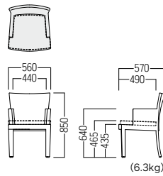
●S・CG-310・AC ㊦ ¥49,500
